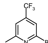
2-Bromo-6-methyl-4-(trifluoromethyl)-pyridine [451459-17-9]
