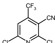
2,6-Dichloro-4-(trifluoromethyl)-pyridine-3-carbonitrile [13600-42-5]
