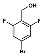
4-Bromo-2,6-difluorobenzyl alcohol [162744-59-4]
