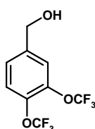
3,4-Bis(trifluoromethoxy)benzyl alcohol [ --- ]
