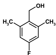
4-Fluoro-2,6-dimethylbenzyl alcohol [773868-67-0]
