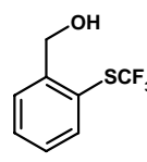
2-(Trifluoromethylthio)benzyl alcohol [239463-93-5]
