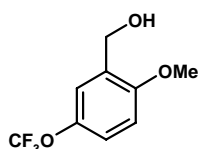
2-Methoxy-5-(trifluoromethoxy)benzyl alcohol [562840-50-0]
