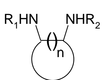
cyclic diamine
