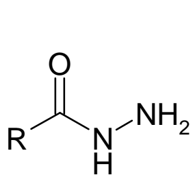
acid hydrazide
