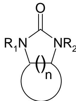
cyclic ureas
