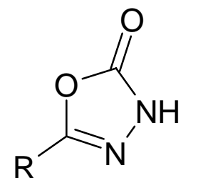
oxadiazolines
